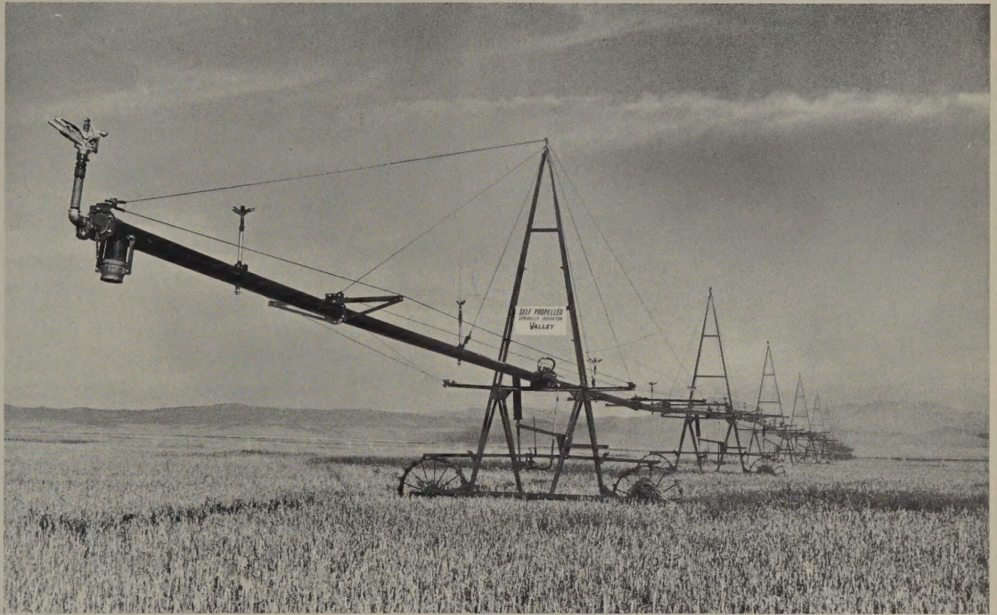
(Above) This mechanical giant is a self-propelled sprinkler system, a modern method of bringing water to land which could not otherwise be cultivated.
